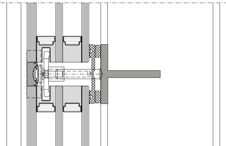
VISS Basic Semi SG Width 50 mm Welding stud
