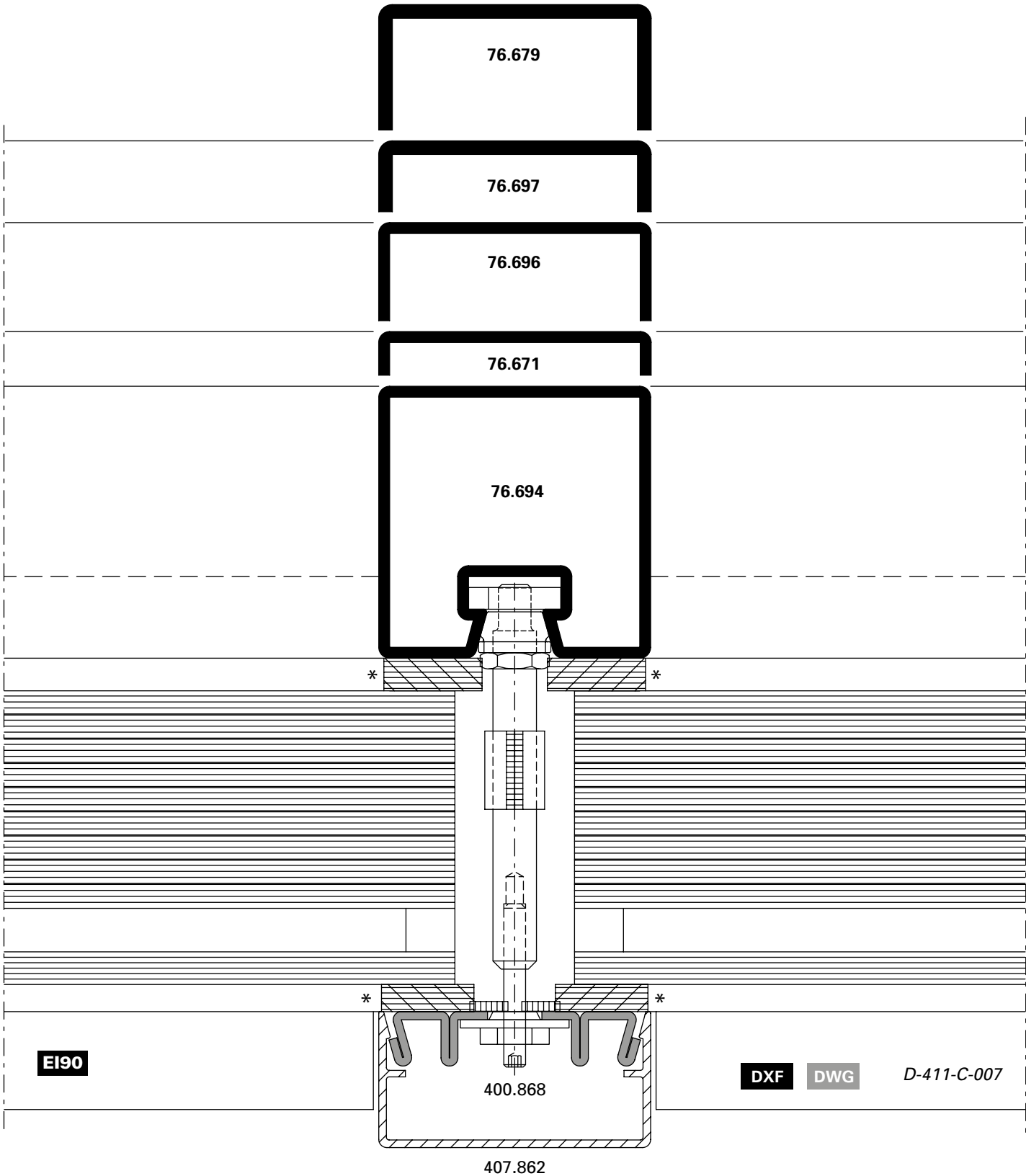
Pfosten-Detail
