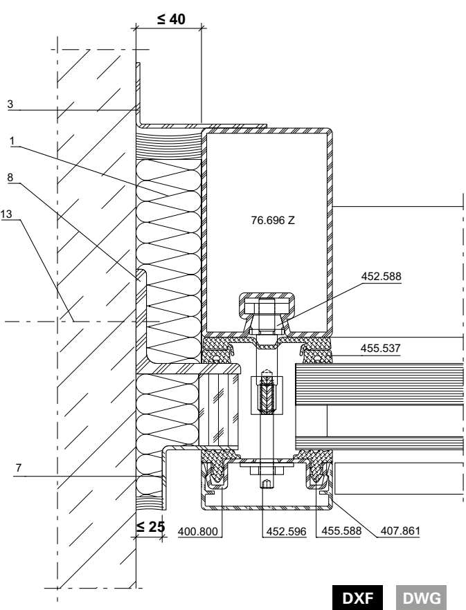
Wall attachment
