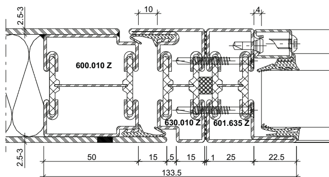
DXF DWG 11-0109-K-001
