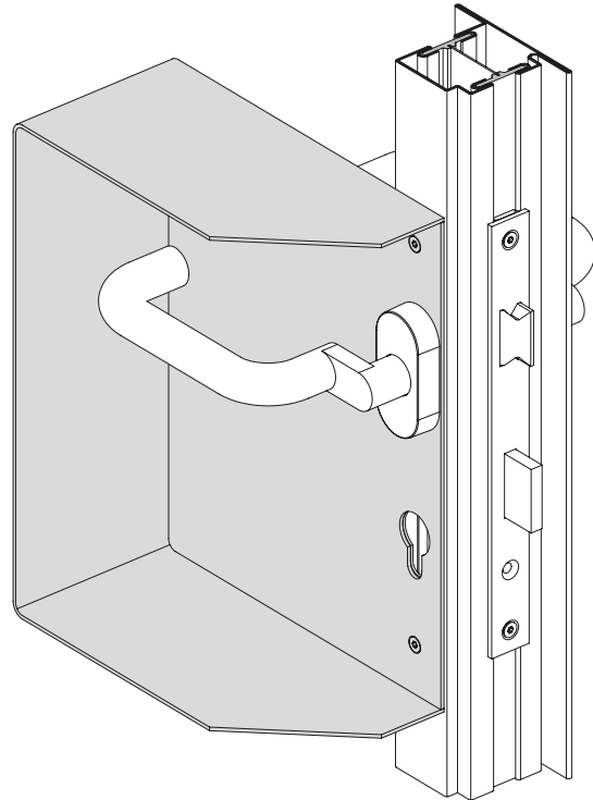
Schutzhaube Capot de protection Protective cover
