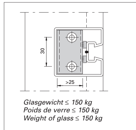
T-connectors screwed, transom push-fitted
