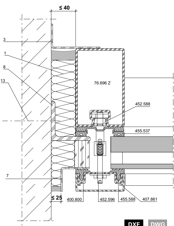
Wall attachment
